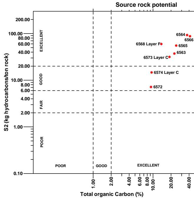
Figure 3. Even though lignites in the Tjörnes beds are thermally immature, they show great potential for source rock, given the proper circumstances. This organic substance can very well be the source of the gases found in Öxarfjörður.
