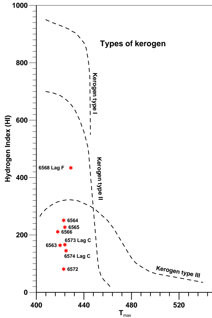
Figure 2. A graph which indicates the type of kerogen found in lignites from the Tjörnes horst, extracted from T_{max} and HI. The T_{max} (420–430°C) indicates that the samples are thermally immature. Vit.ref. of 0.25–0.3 supports that. At least one sample consists possibly of more than terrestrial material, and even some of the other as well.
