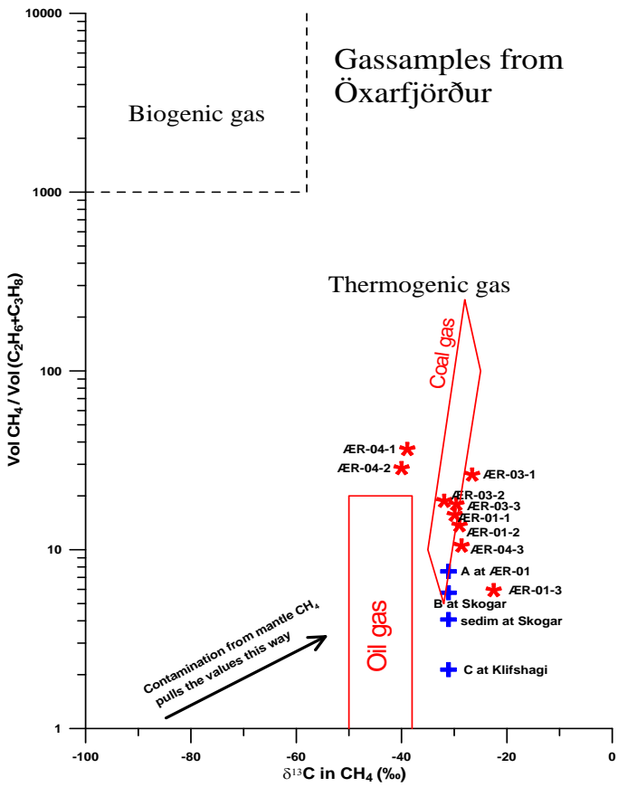
Figure 4. Analyses made in 1999 (blue crosses) as well as analyses done 12 years ago (red stars). The gas is without doubt thermogenic and not biogenic. Since this is a volcanic region, it may be possible that methane from magma could contaminate the samples, shifting them towards the right and up. If that is so, many of the samples could actually have lower \delta^{13}\text{C} (mantle methane has \delta^{13}\text{C} > -10 ). Blue crosses have a \delta^{13}\text{C} mean value extracted from the older data. The value from the result of the analyses of Muelenbachs, indicates that the blue crosses should be shifted to approximately -25 \delta^{13}\text{C} .
